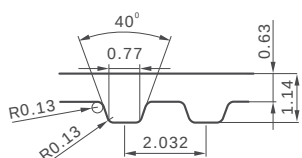
MXL (Rubber)
