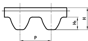
Eagle profile 8M - 14M
