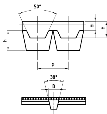
ATK5-K6 ATK10-K13
