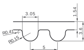
HTD 5M (Rubber)
