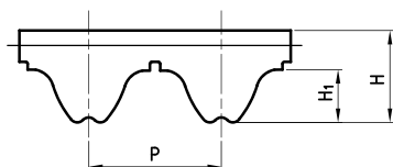
RTD 5M - RTD 8M - RTD 14M RTD 14M XHPL
