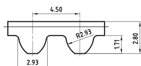
STD 4,5M (Rubber)
