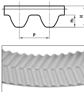
EAGLE 8M - EAGLE 14M
