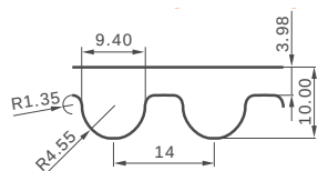
HTD 14M (Rubber)
