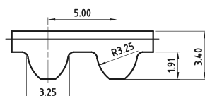
STD 5M (Rubber)
